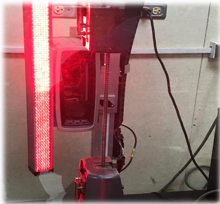
Conducting a Rebar Tensile Test at TTBS Lab
